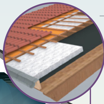
Roof insulation
